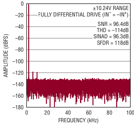
32k Point FFT f_{SAMPL} = 200\text{kHz} , f_{IN} = 2\text{kHz}
