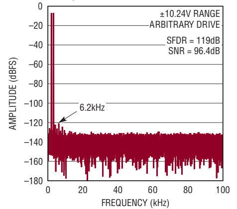
32k Point Arbitrary Two-Tone FFT f_{SAMPL} = 200\text{kHz} , IN^+ = -7\text{dBFS } 2\text{kHz} Sine, IN^- = -7\text{dBFS } 3.1\text{kHz} Sine
