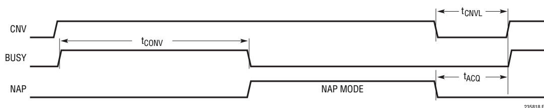
Figure 13. Nap Mode Timing for the LTC2358-18
